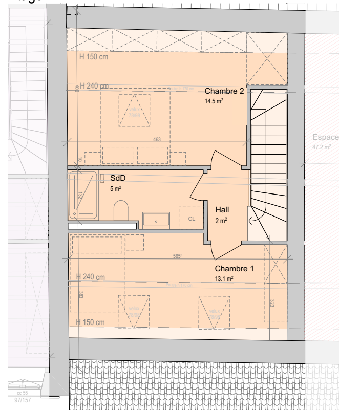
Combles
